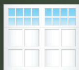
I108S
