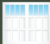
I204S
