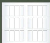
I300S
