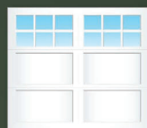
I006S
