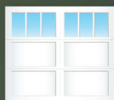
I003S
