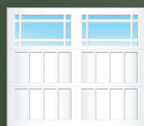
I309S
