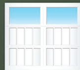
I301S
