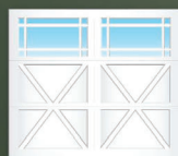
IX09S
