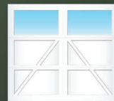
IA01S
